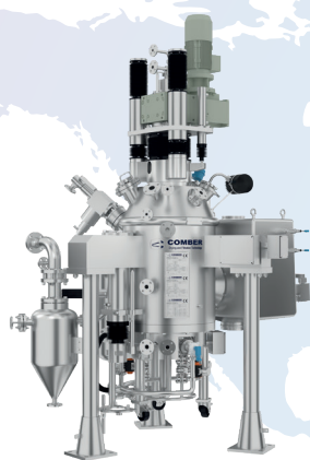
PRESSOFILTRO® Filterdryer / Agitated Nutsche Filter
